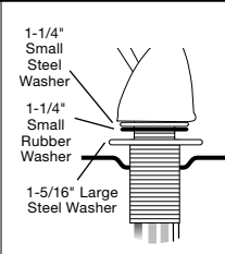
Standard 1-1/2" hole
